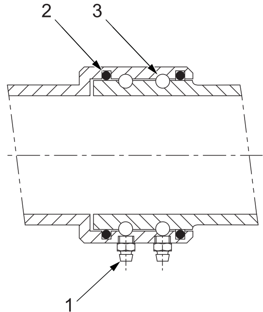
Figure 2. Section showing details of bearings
